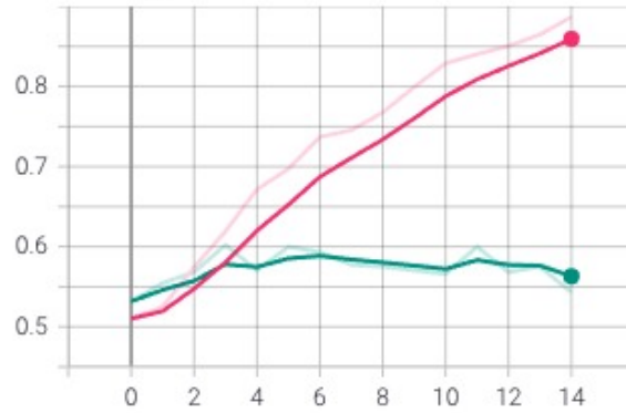
Figure 4: Experiment 1 Accuracy as a Function of Epoch Number
