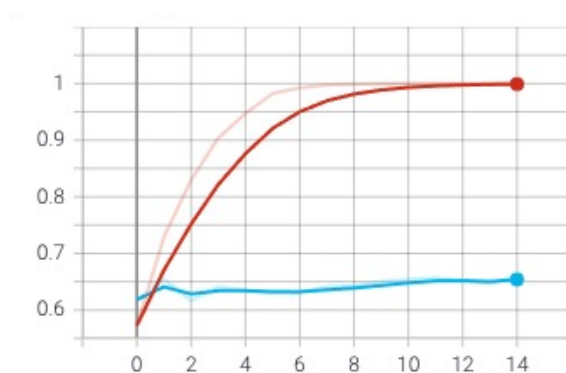
Figure 8: Experiment 2 Accuracy as a Function of Epoch Number
